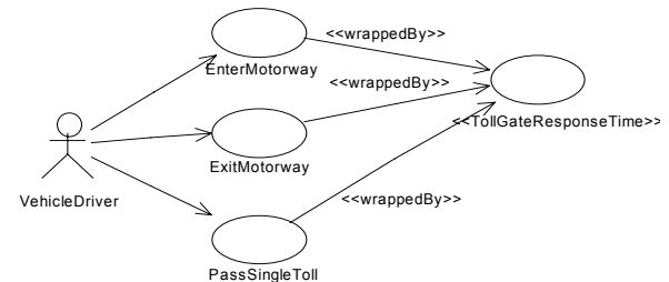
Figure 4. A use case composed with an aspect
