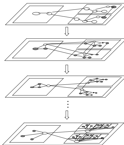
Figure 11 Architectural Levels
