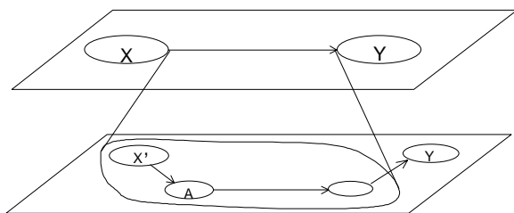
Figure 12. Interaction Refinement
