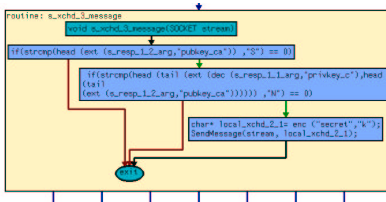
Fig. 7. Control graph for s_xchd_3_message function
