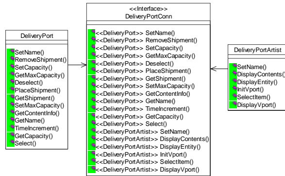
Fig. 8. Interface class for the DeliveryPortConn connector
