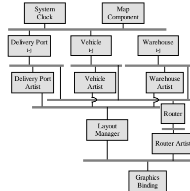
Fig. 4. C2 Architecture of the Cargo Routing System
