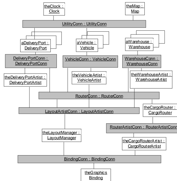
Fig. 9. Collaboration diagram representing instances of internal objects
