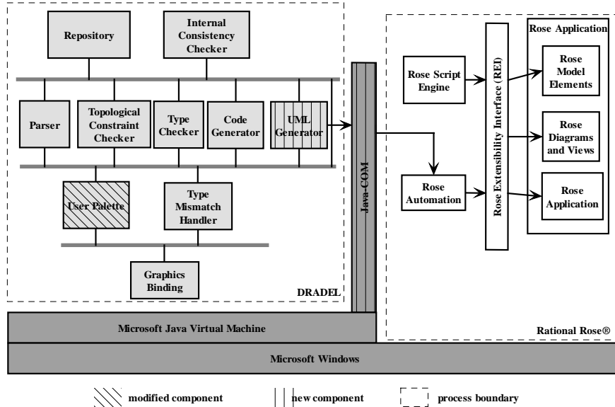
Fig. 11. Architecture of the integrated environment. DRADEL and Rose are running in separate processes and communicating through synchronous COM remote procedure calls
