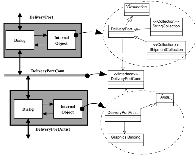
Fig.7. Designing the Internal Object. Artist, Destination, ShipmentCollection, StringCollection are not part of the transformation, but were added manually by the designer.
