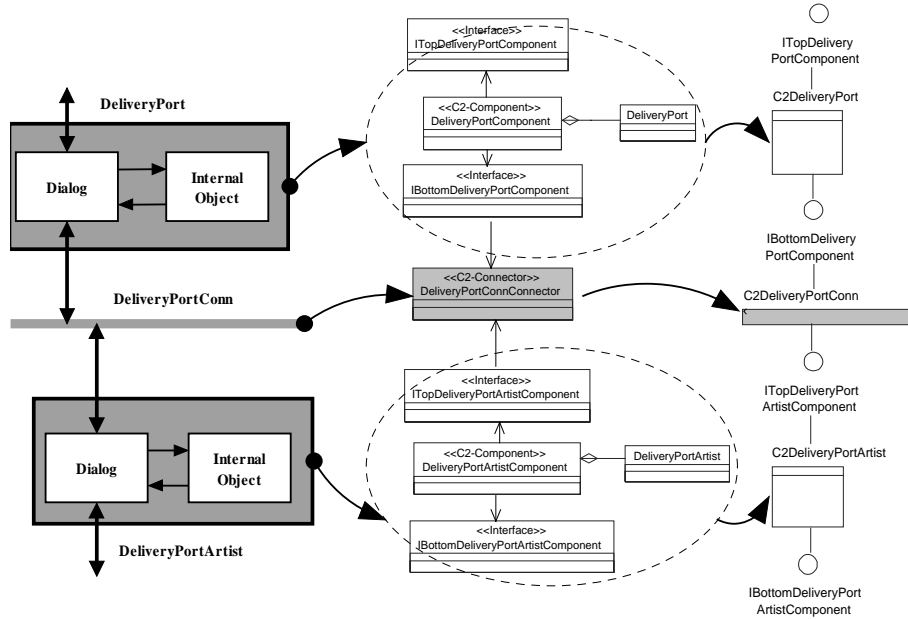
Fig. 10. Representing Architectural Constructs in UML. Of course, the C2 component has to realize the classes added by the designer to represent the internal object (not shown here)
