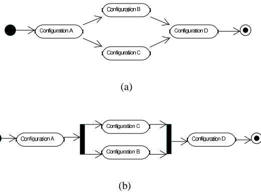
Figure 6: Modeling nondeterministic mobility behavior 6(a) and mobile concurrent execution of multiple agent instances 6(b)
