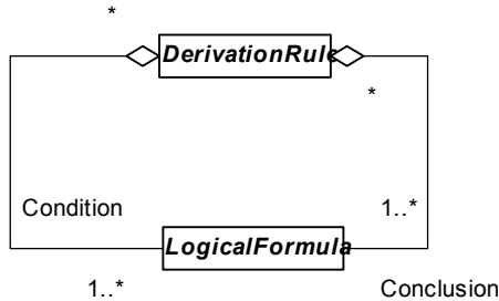
Figure 2: The general format of derivation rules.
