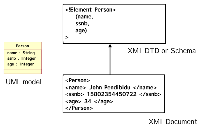
Figure 3: XMI representation of MOF-compatible models
