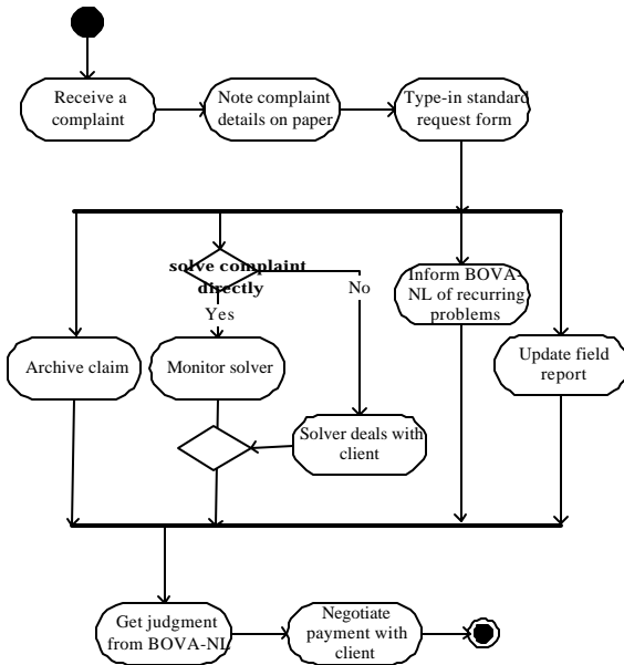
Figure 3. Activity Diagram Specification of the Task "Handle a Complaint".
