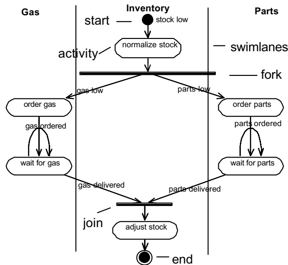
FIG. 13. An activity diagram.
