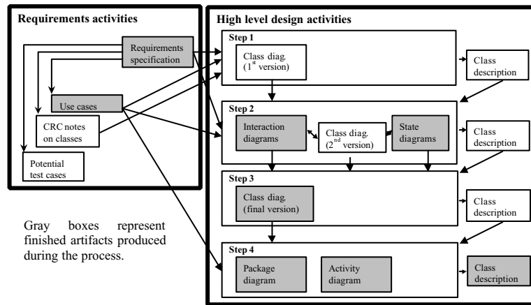
FIG. 2. High-level design activities, using artifacts created during the requirements phase and during PBR requirements inspections.
