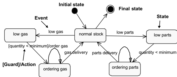
FIG. 10. A statechart.
