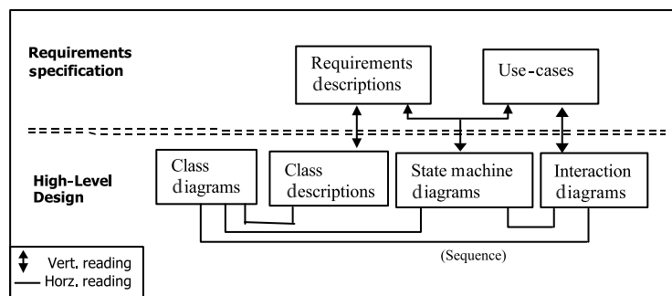
FIG. 4. The set of OORTs (each arrow represents one technique) that has been defined for various design artifacts.
