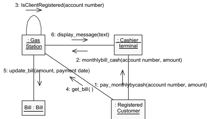
FIG. 9. A collaboration diagram.
