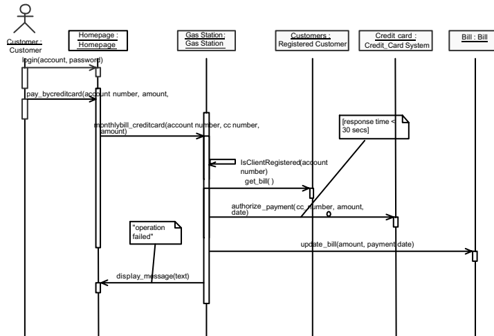
FIG. 20. Sequence diagram.
