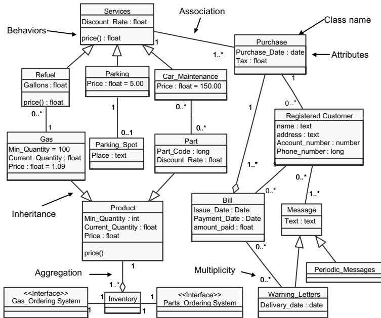
FIG. 6. An example of a UML class diagram.
