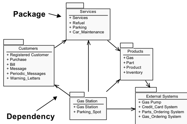
FIG. 12. An example of a package diagram.
