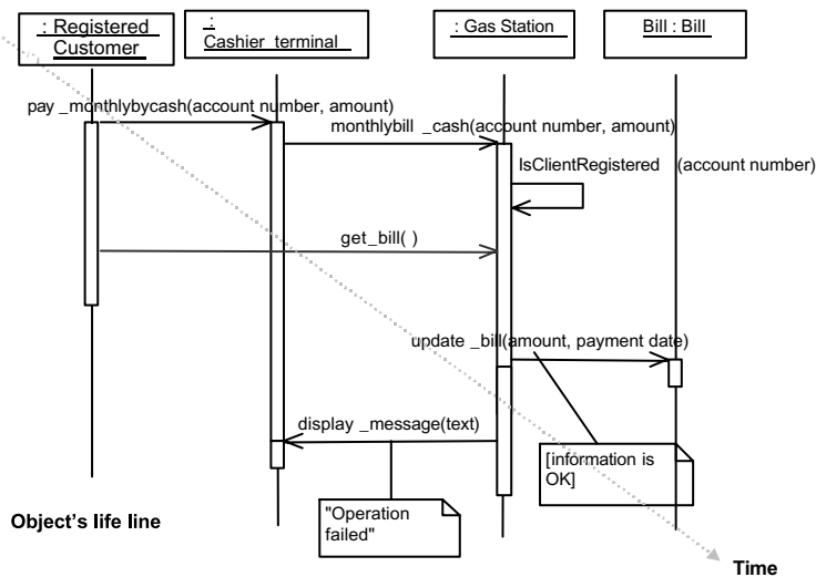
FIG. 8. An example of a sequence diagram.
