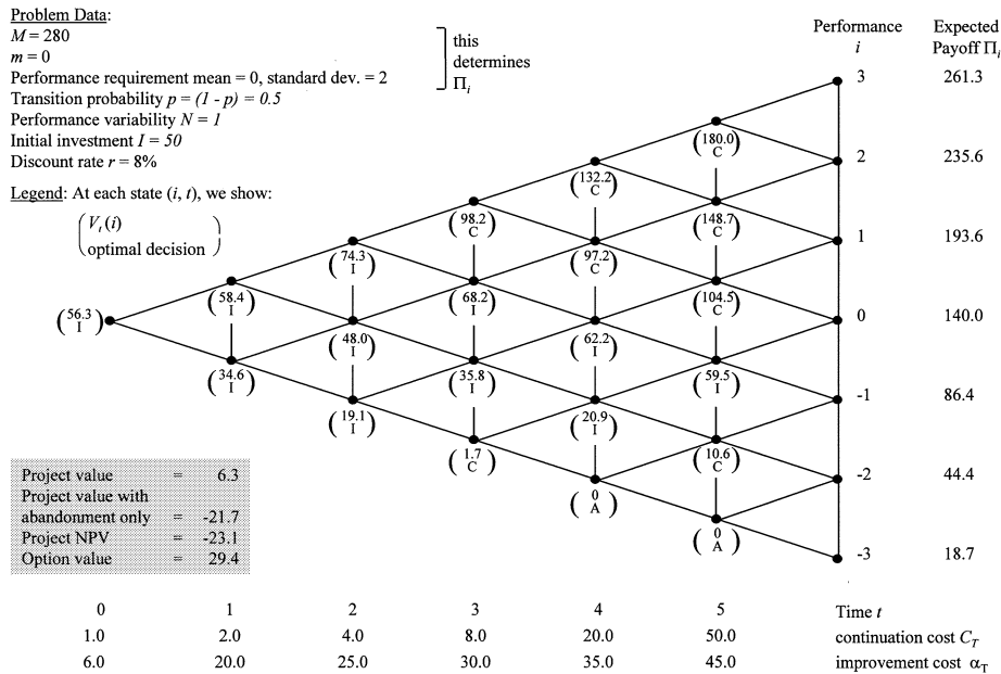
Figure 5 Example of Optimal Policy and Value Function
