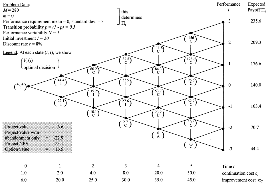
Figure 8 Example with Increased Requirements Variability
