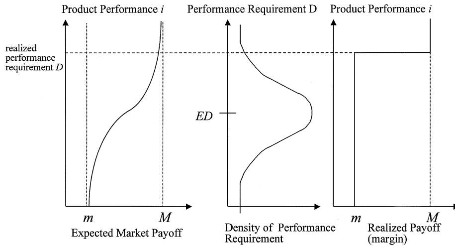
Figure 3 Market Uncertainty and Project Payoffs
