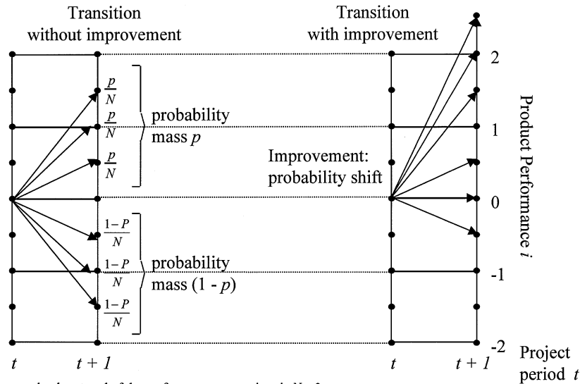
Figure 2 Transition Probabilities of Product Performance
