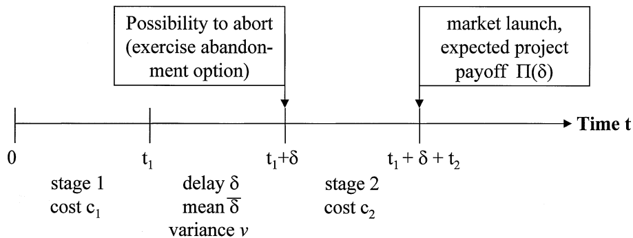
Figure 9 A Development Project with Schedule Uncertainty
