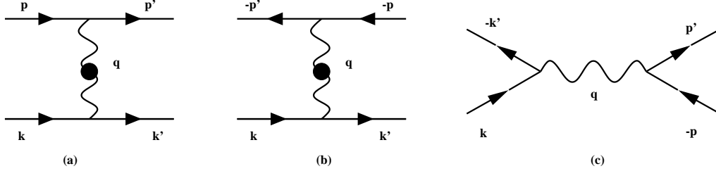
Figure 7: Scattering processes described by the collision term in eq. (2.73) : (a) particle-particle scattering; (b) particle-antiparticle scattering ( t -channel); (c) particle-antiparticle annihilation ( s -channel). In Fig. (c), the virtual photon is always hard, so it needs no resummation.
