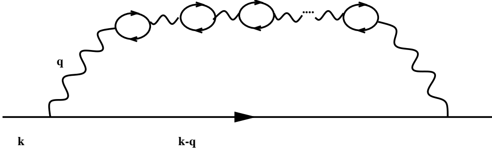
Figure 5: One of the multi-loop diagrams (containing n bubble insertions along the photon line) which is included in the effective one-loop diagram in Fig. 4.
