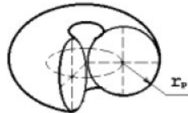
Figure1. Electron model
